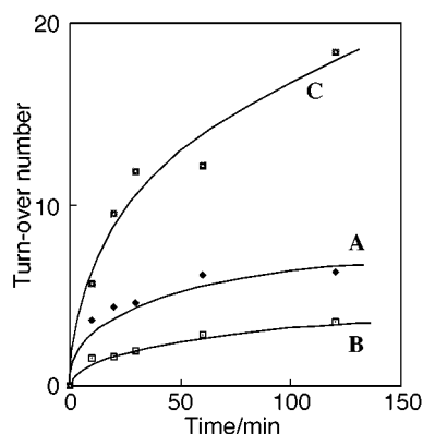
Fig. 4 Plots of turnover numbers (= [mole of product]/[mole of iron(III) complex]) of the products catalysed by red [\text{Fe}_2\text{O}(\text{CH}_3\text{CO}_2)_2(\text{tfpy})_2][\text{ClO}_4]_2 \cdot 2.2 : A, cyclohexanol; B, cyclohexanone; C, cyclohexyl hydroperoxide.
